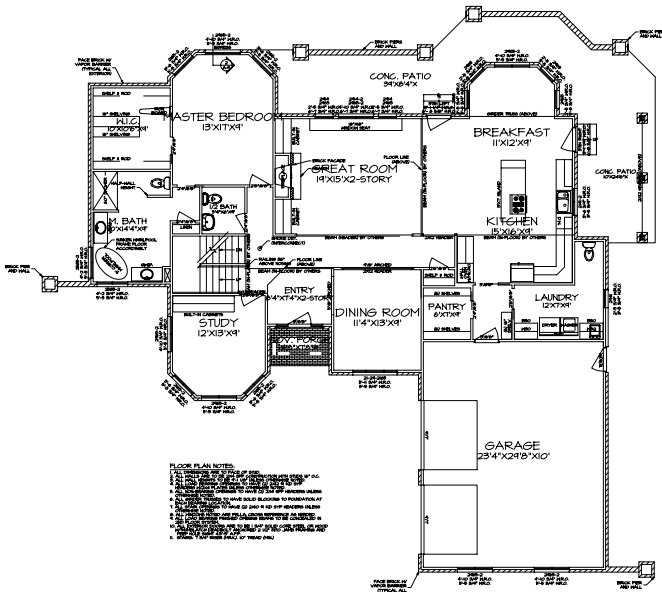
1 FIRST FLOOR PLAN A-3 SCALE: 1/4"=1'-0"
