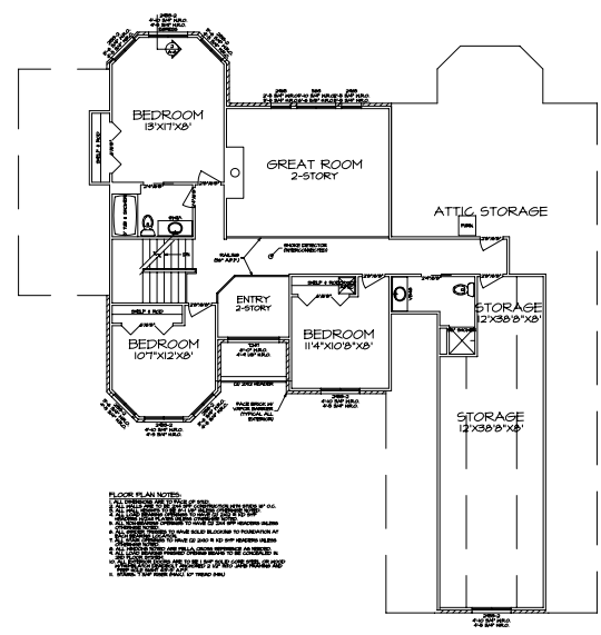
1 SECOND FLOOR PLAN A-6 SCALE: 1/4"=1'-0"
