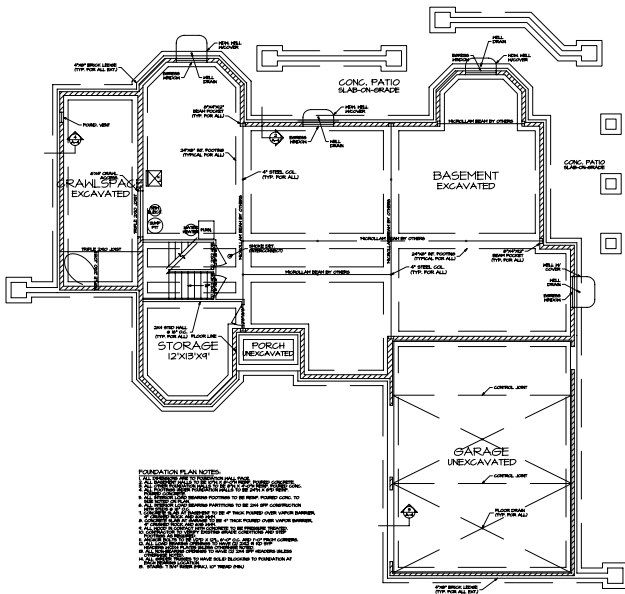
1 FOUNDATION PLAN A-2 SCALE: 1/4"=1'-0"
